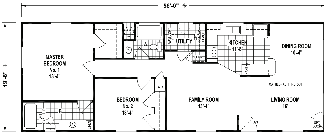
4616CTC/5620 (1,101 SQ. FT.) 2BEDROOM - 2BATHS - CATHEDRAL THRU-OUT
